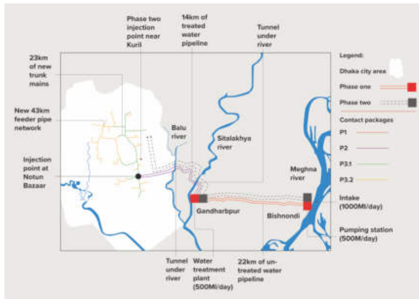
Figure 2.1: Source- Surface water treatment and transmission
